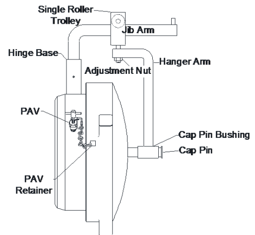
Horizontal 16-24 300" drawing
